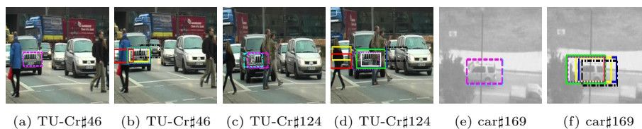
Fig. 4: Tracking through multiple partial occlusions. MTS-TS(magenta), MTS-L(cyan), SCM(green) FragT(white), Semi(yellow), L1-APG(blue), VTD(red), WLMCMC(black), and ASLA(purple).
