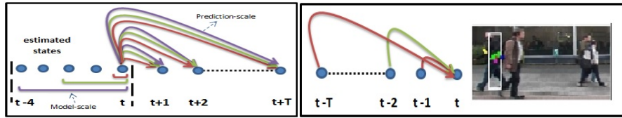
(a) Multiple motion models are learned from the recent history of estimated states at different temporal scales, and each model is applied to multiple temporal scales in the future.
